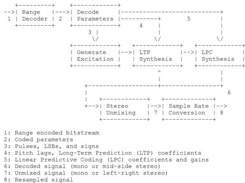
Figure 14: SILK Decoder
