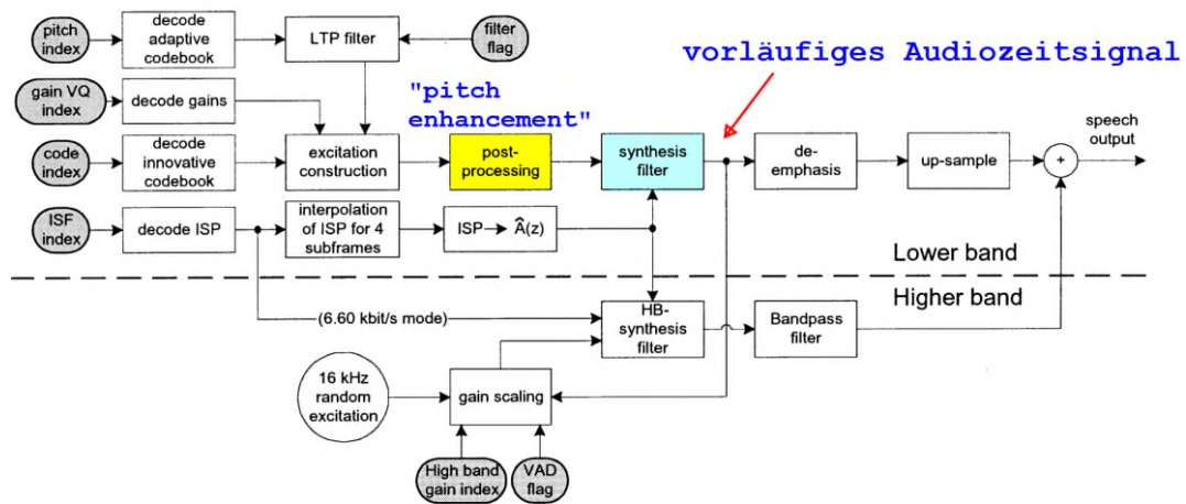
Fig. 2. Block diagram of the AMR-WB ACELP decoder.
